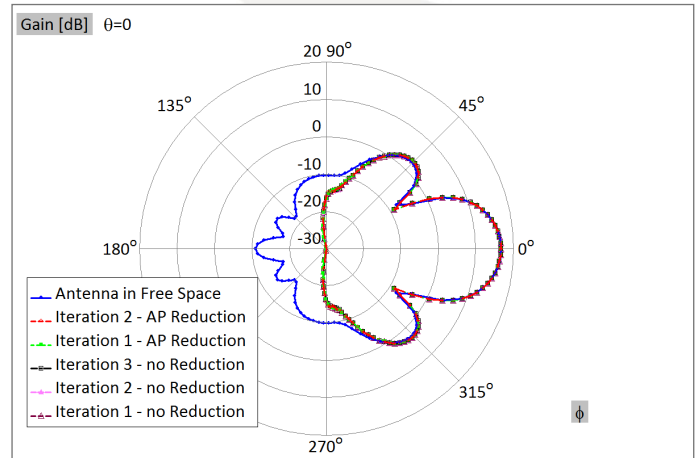
Figure 5. Radiation patterns of the anti-collision radar antenna in free space and anti-collision radar antenna mounted on the bumper
