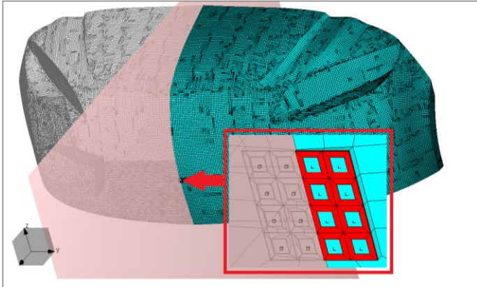
Figure 3. Anti-collision radar antenna mounted on the bumper – WIPL-D Pro
