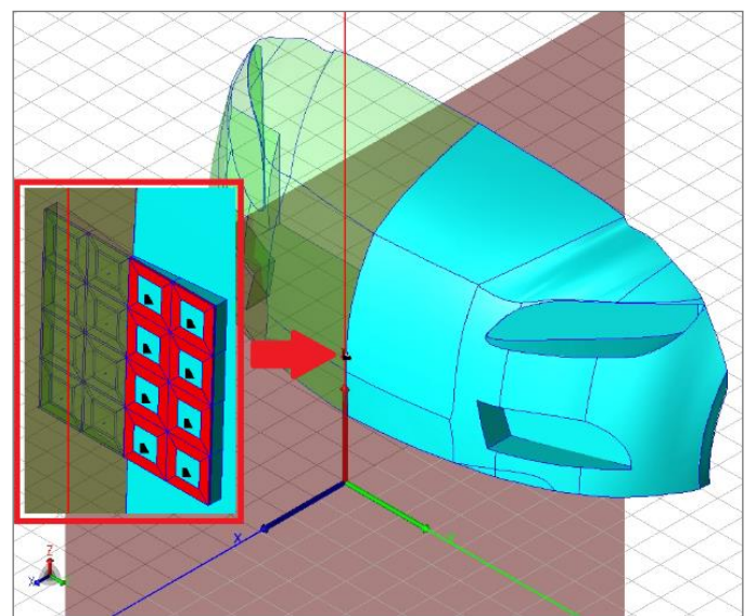
Figure 2. Anti-collision radar antenna mounted on the bumper – WIPL-D Pro CAD
