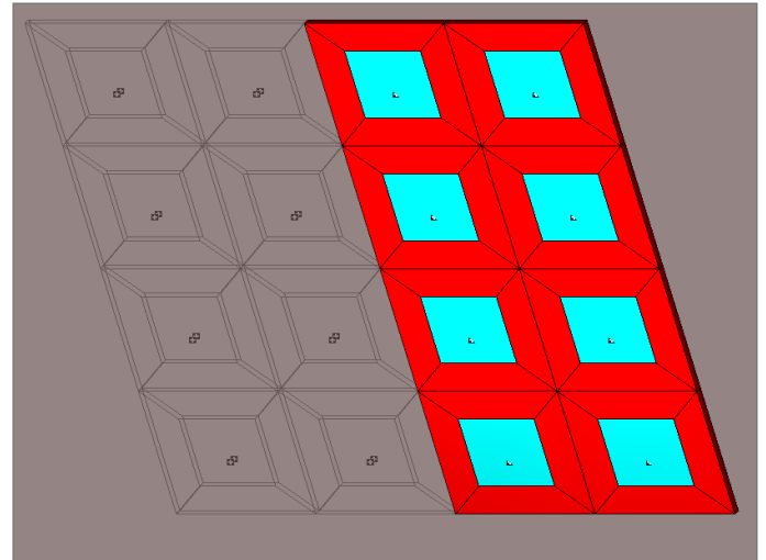
Figure 1. Anti-collision radar antenna – WIPL-D Pro
