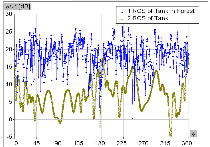
RCS of Tank (yellow) and Tank in Forest (blue)
