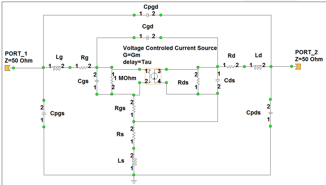
Figure 1. Equivalent circuit model of low power GaAs HEMT transistor implemented in WIPL-D Microwave.
