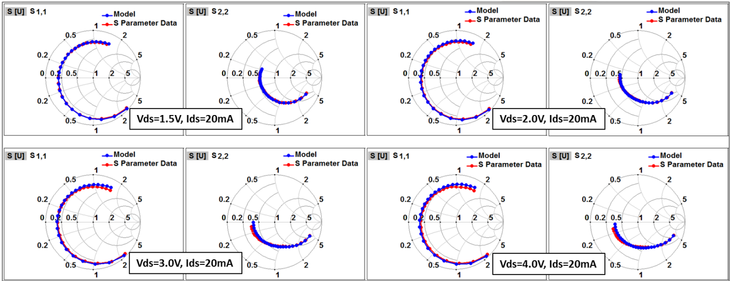
Figure 3. Comparison of S11 and S22 obtained by measurements and transistor model presented in Fig. 1 for four Vds values.
