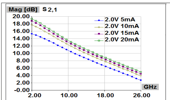
Figure 5. Variations of S21 with Ids for Vds=2V.
