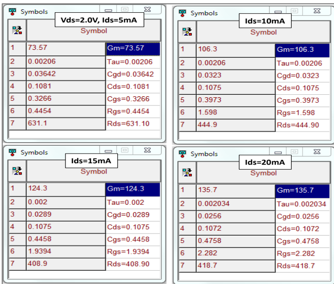
Figure 4. Four sets of values for intrinsic transistor model elements used to study the variation of S21 with Ids for Vds=2V.
