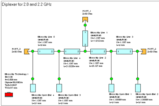
Figure 3. Diplexer
