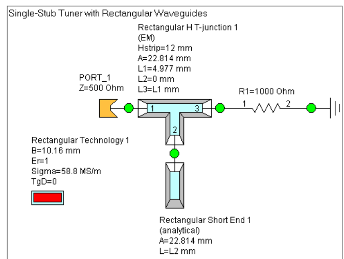
Figure 1. Single-stub tuner with rectangular waveguides
