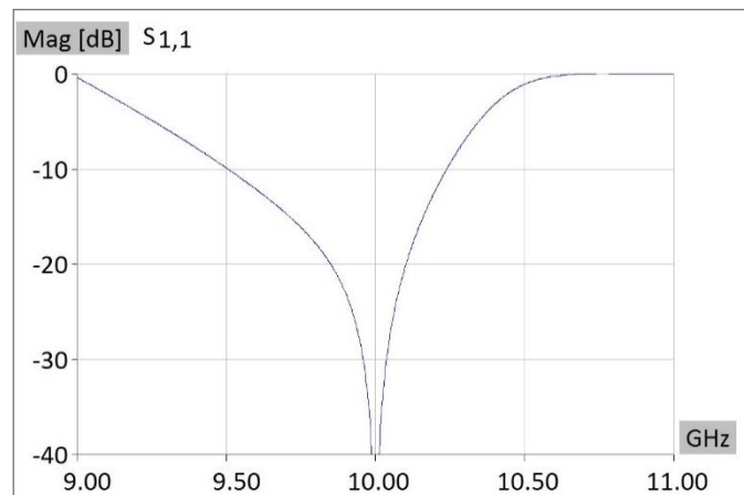
Figure 2. Parameter s11 for circuit shown in Figure 1.
