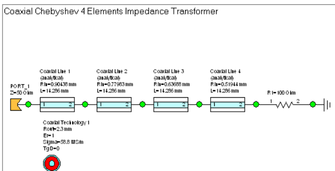
Figure 5. Coaxial Chebyshev impedance transformer
