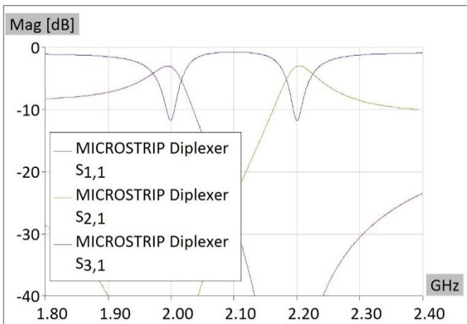
Figure 4. S parameters for network shown in Figure 3.
