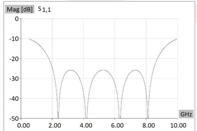
Figure 6. Parameter s_{11} for network shown in Figure 5
