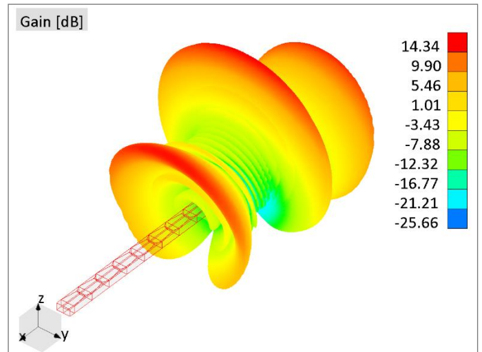
Fig.7. Radiation pattern of the array
