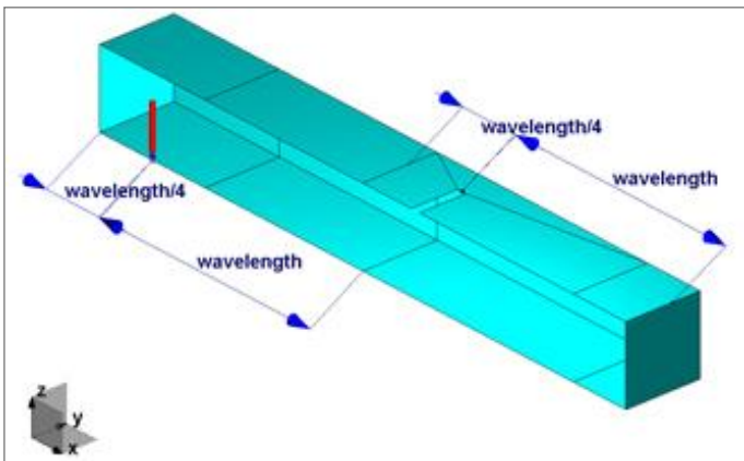
Fig.1. Model of one waveguide slot – one symmetry plane
