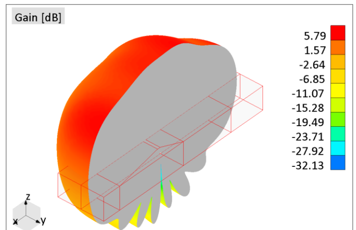
Fig.4. Radiation pattern in half-space of a single slot
