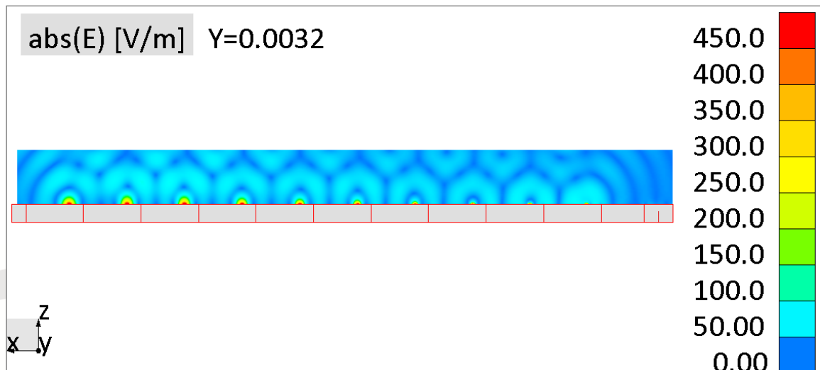
Fig.7. Radiation pattern of the array
