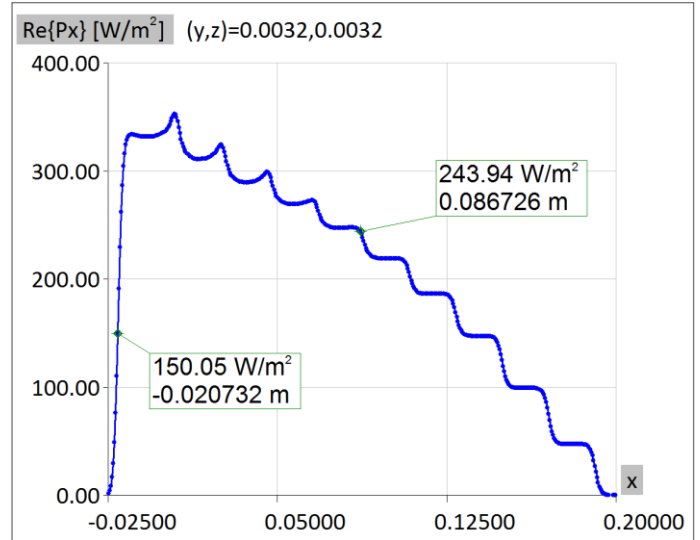
Fig.6. Real part of the Poynting vector longitudinal component along the axis of the waveguide (array)
